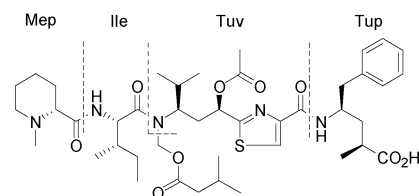
Figure 1. Tubulysin D ( 1 ).
